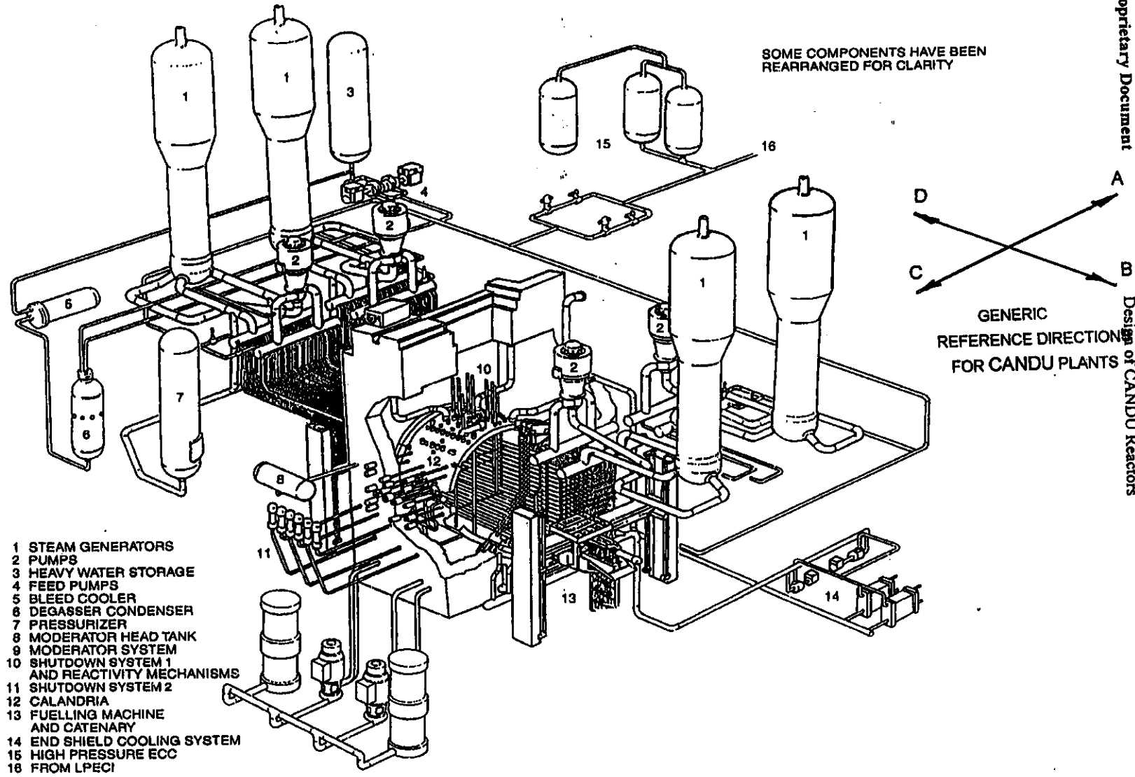
Figure 1-6 Cutaway View of CANDU NSSS
