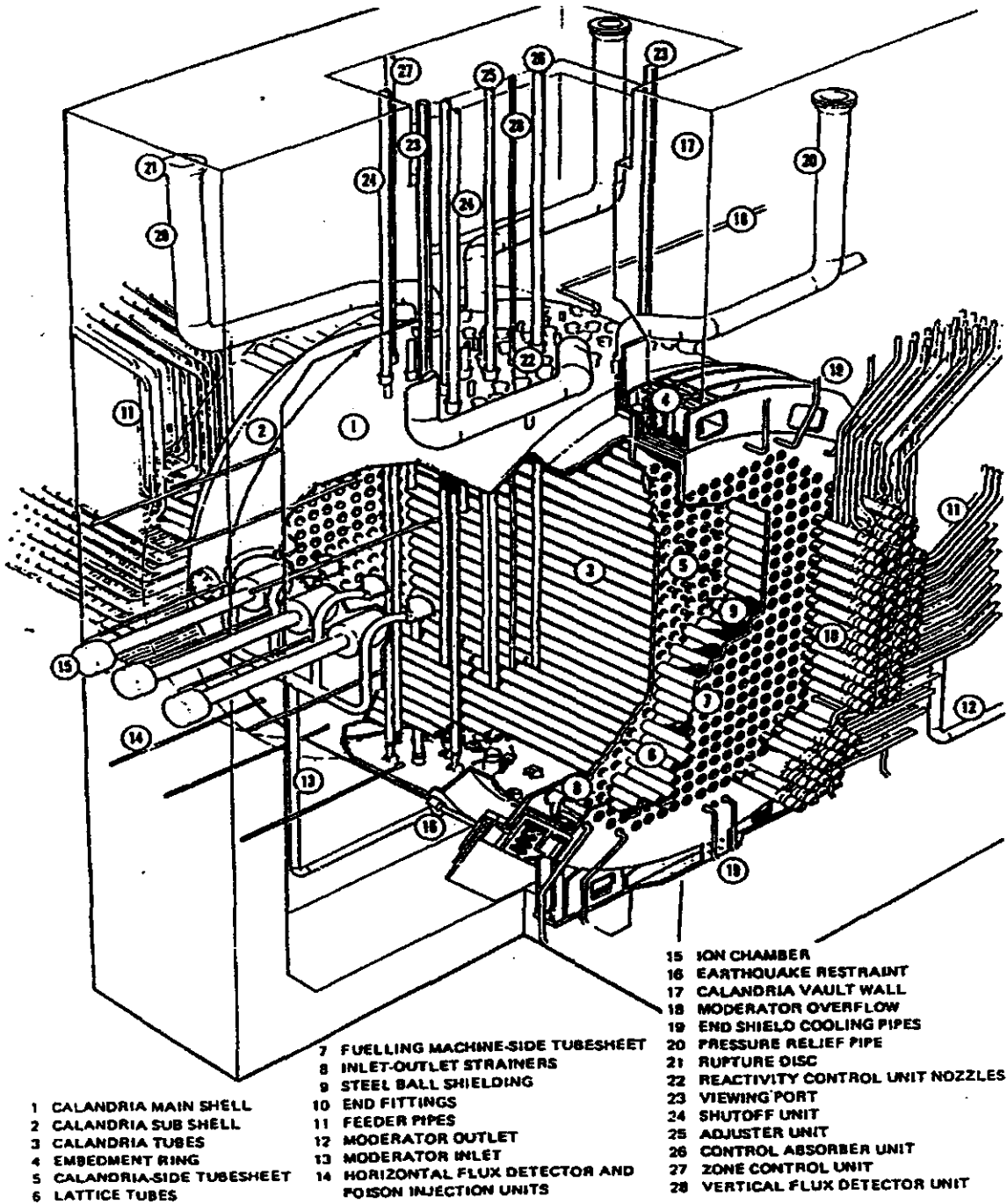
Figure 1-5 CANDU 6 Reactor and Vault Assembly
